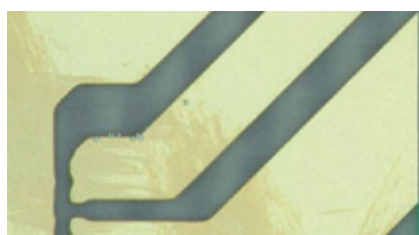
炉前锡球 Pre-reflow solder ball
